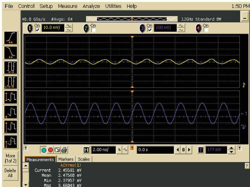
Figure 7. Scope triggered on sine wave, using averaging
