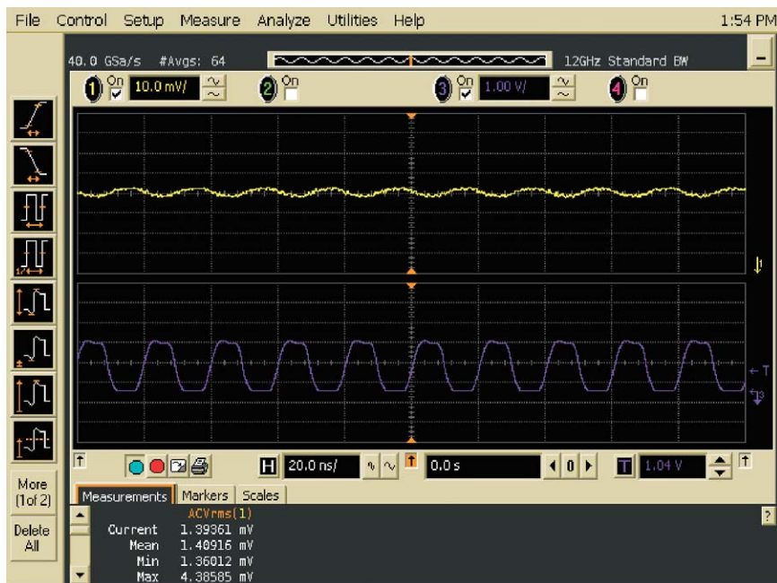
Figure 8. Scope triggered on square wave, using averaging
