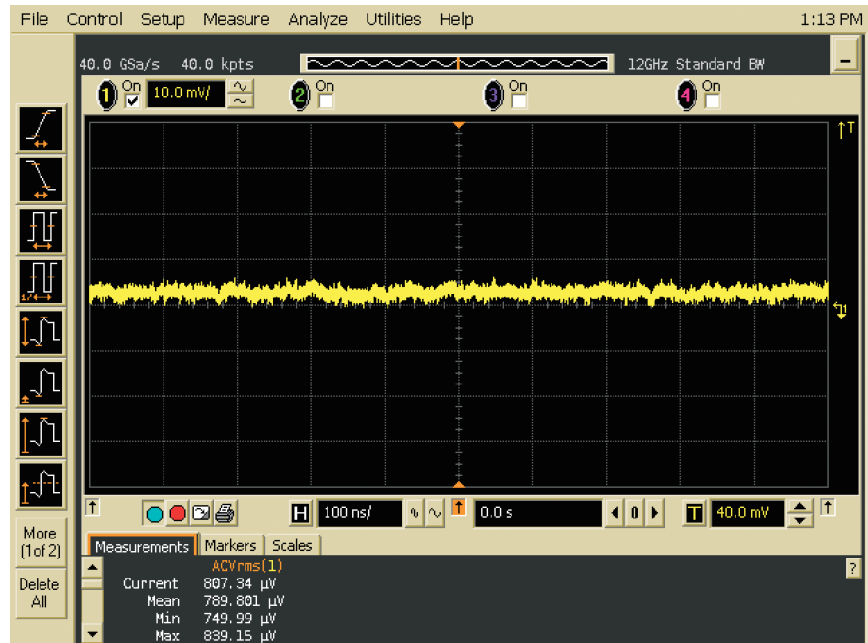
Figure 3. Scope and probe noise
